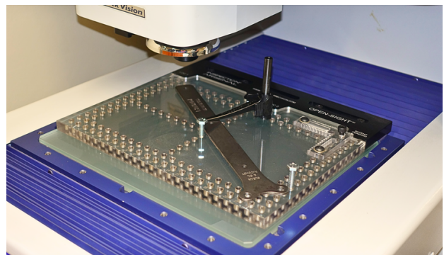
Lowell's Custom Quality Control Optical Measurement Fixtures
